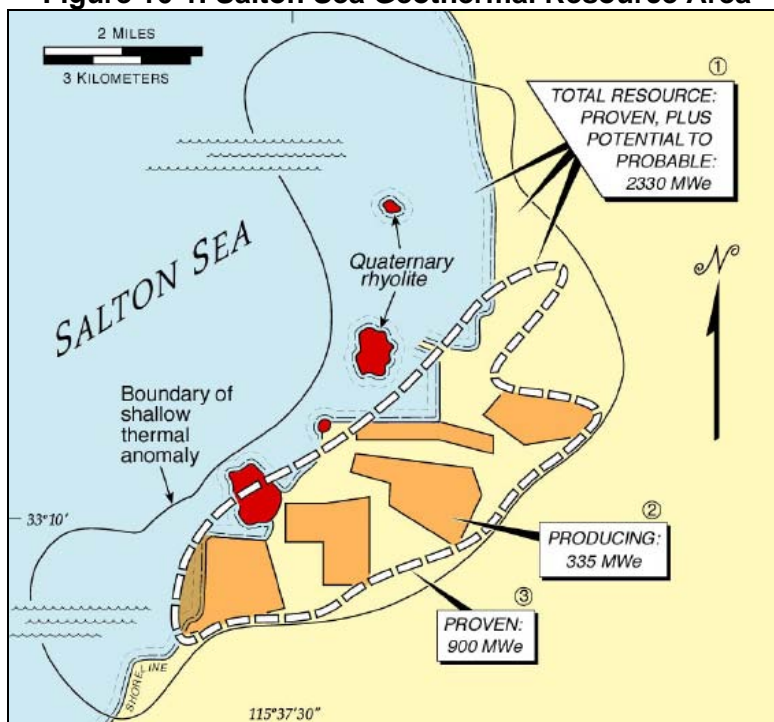
Figure 16-1. Salton Sea Geothermal Resource Area
